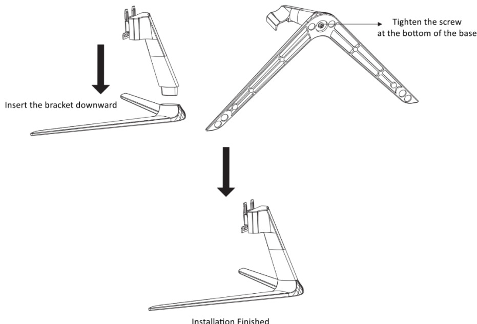
Figure 2-13 Install Bracket and Base (Model A)
