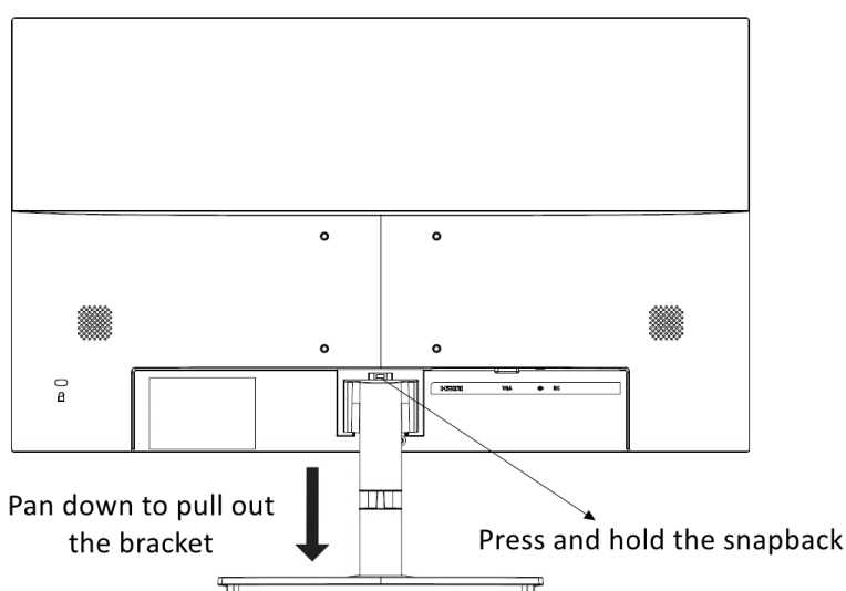
Figure 2-9 Remove the Device and Bracket (Model B)
