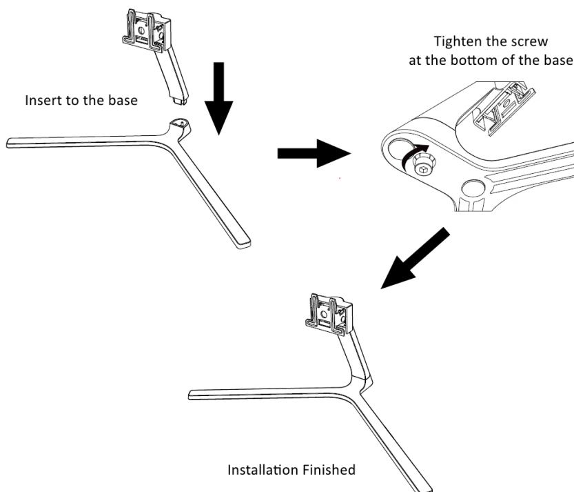
Figure 2-14 Install Bracket and Base (Model B)
