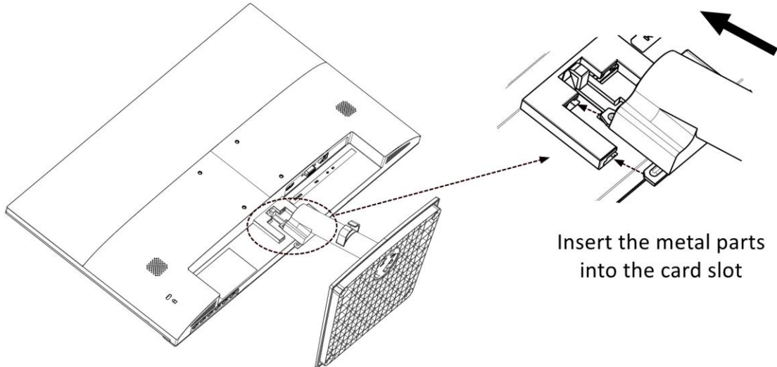
Figure 2-5 Insert the Metal Parts (Model B)
